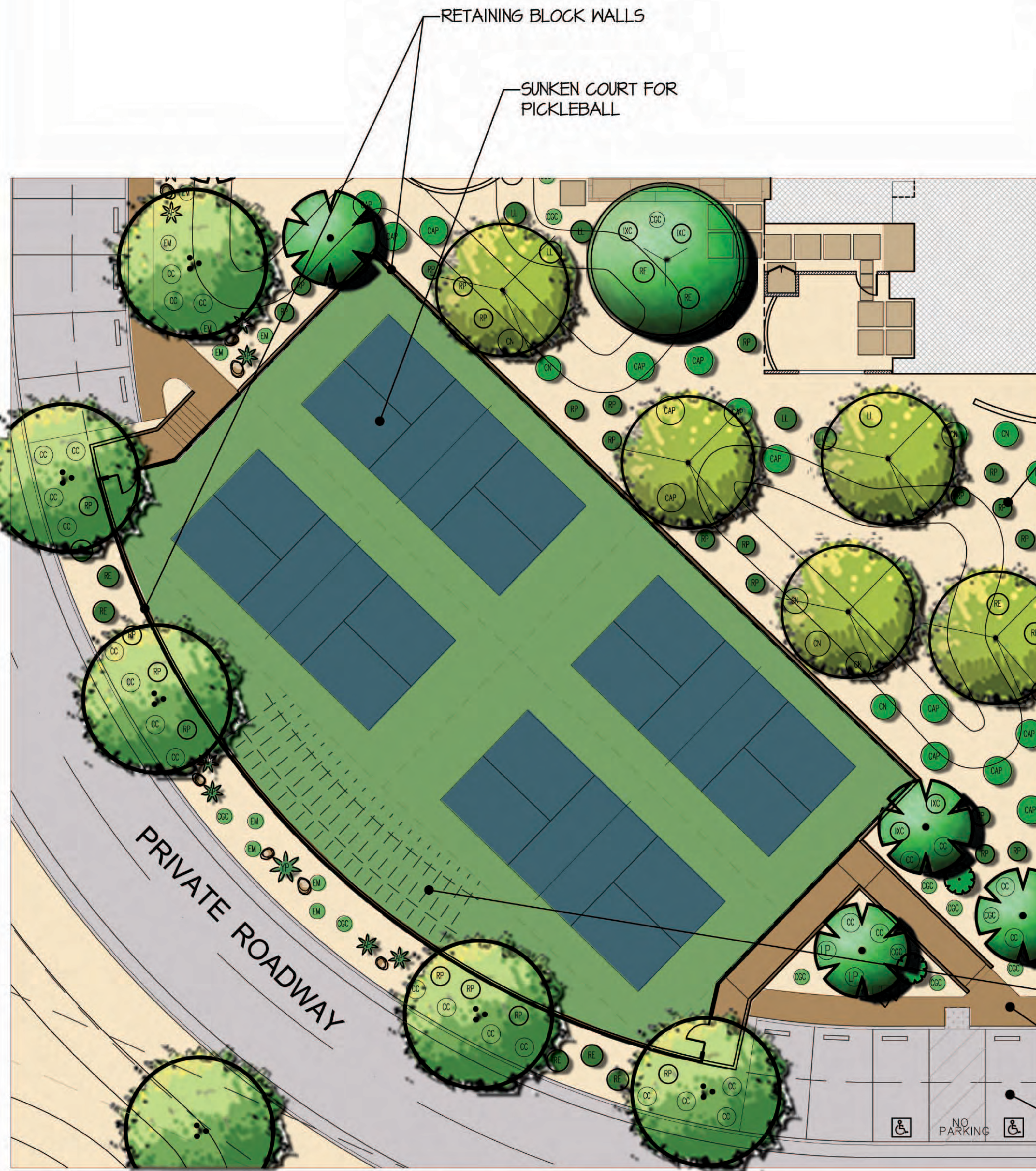
PICKLEBALL COURT EXHIBIT SCALE: 1" = 10'-0"
